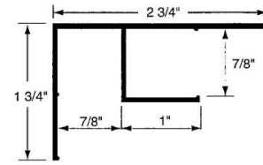
INSIDE CORNER 10'
