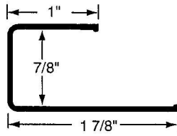
J CHANNEL 12'
